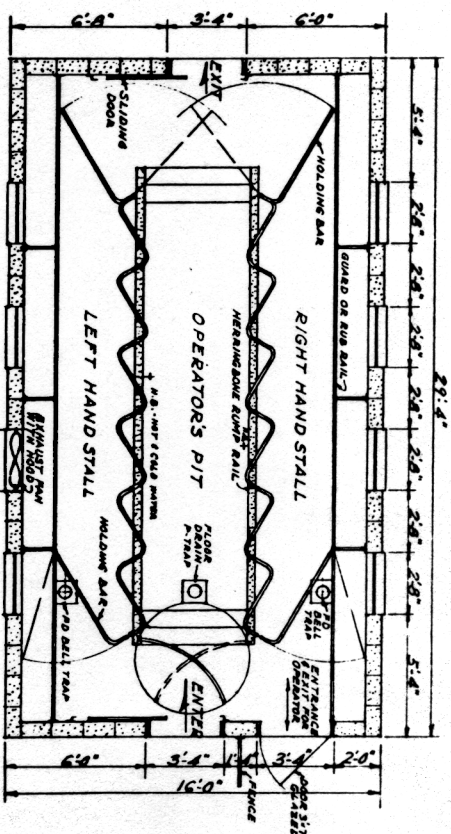
PLAN DOUBLE SIX STALL SCALE: 1/8"=1'-0"
