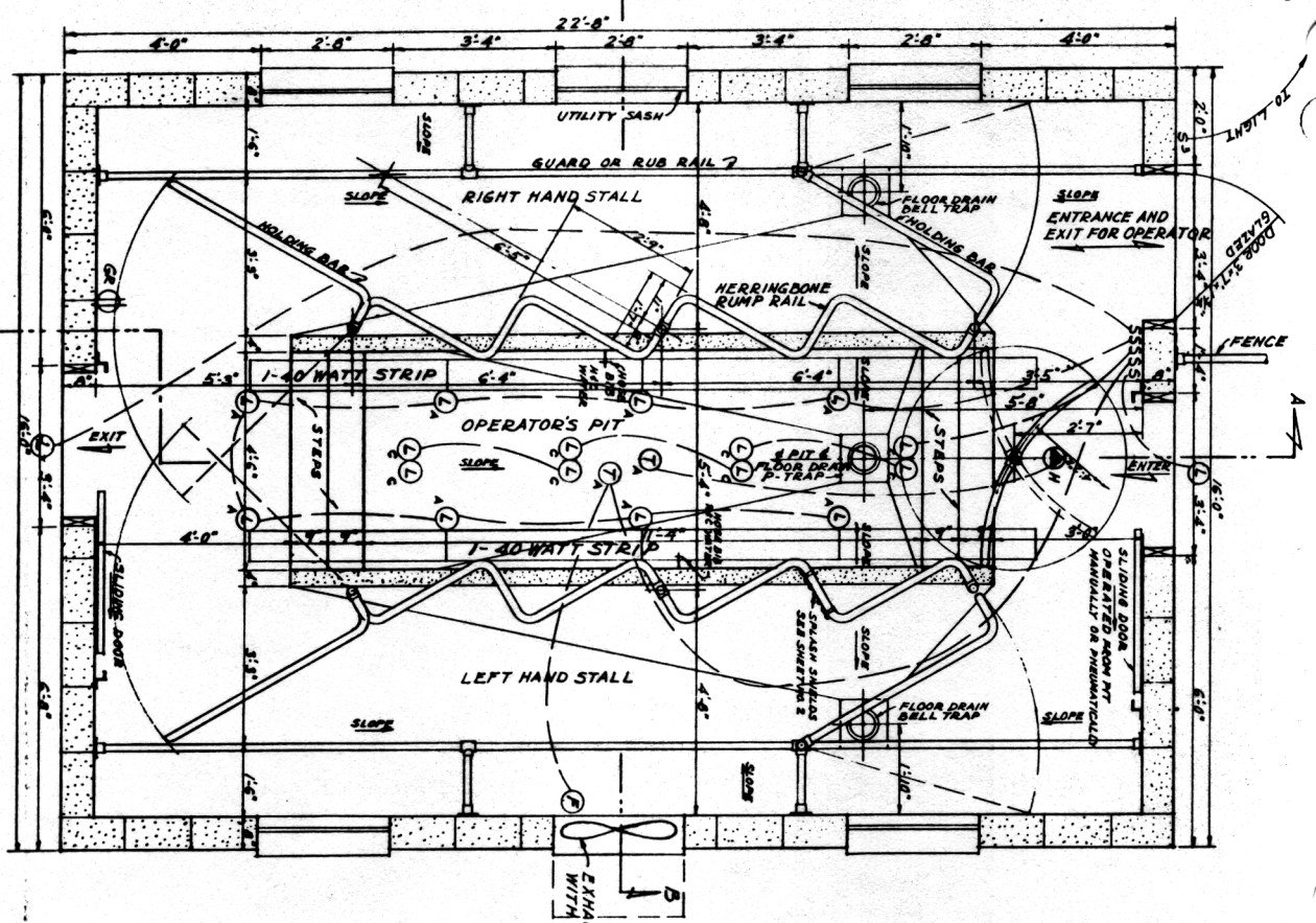
PLAN DOUBLE FOUR STALL SCALE: 1/8"=1'-0"
