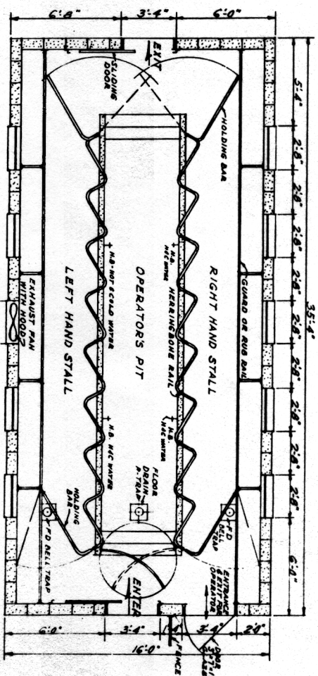
PLAN DOUBLE EIGHT STALL SCALE: 1/8"=1'-0"
