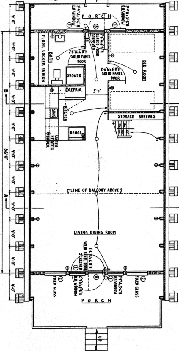
FIRST FLOOR PLAN 0 2 4 6 FT.
