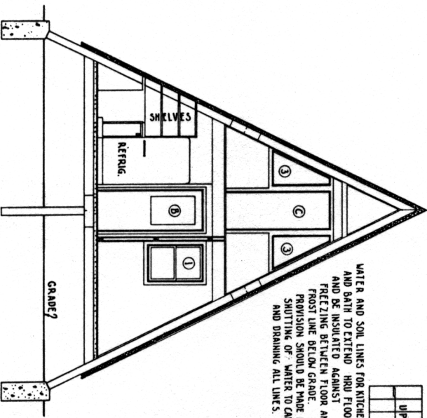
SECTION B-B 0 2 4 6 FT.
