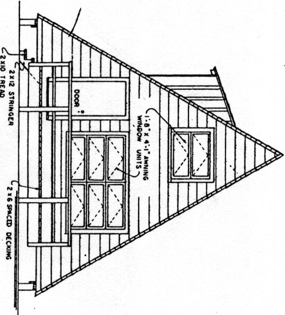
DECK-ENDELEVATION 0 2 4 6 FT.
