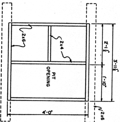
BASE FRAMING PLAN
