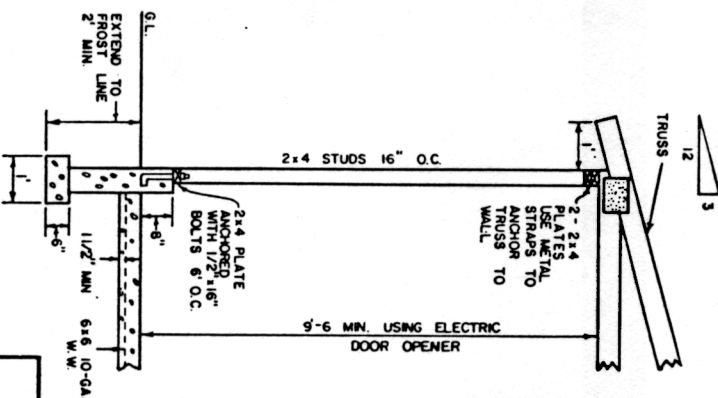
GARAGE CONSTRUCTION NOTES
