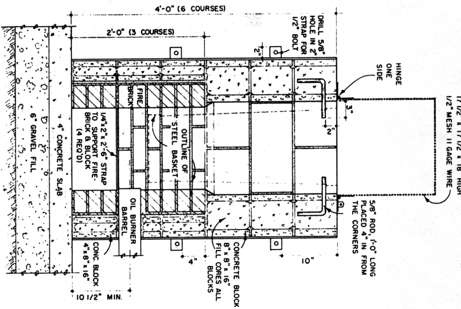
SECTION THRU INCINERATOR
