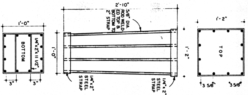
BASKET DETAILS
