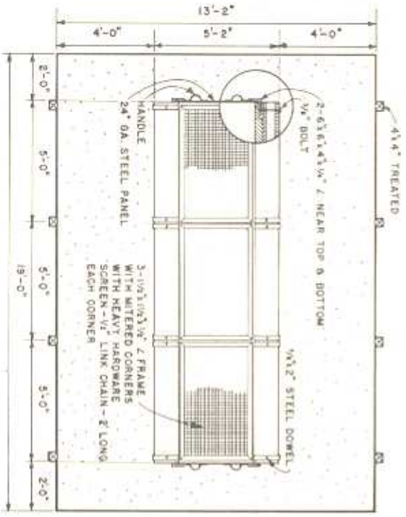
FLOOR PLAN 0 1 2 3 4 FT
