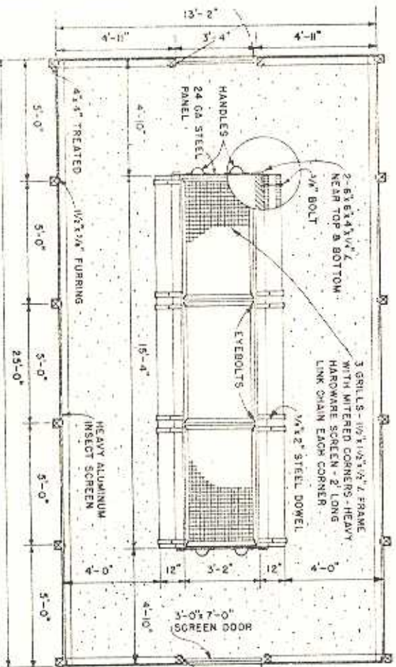
FLOOR PLAN 0 1 2 3 4 FT
