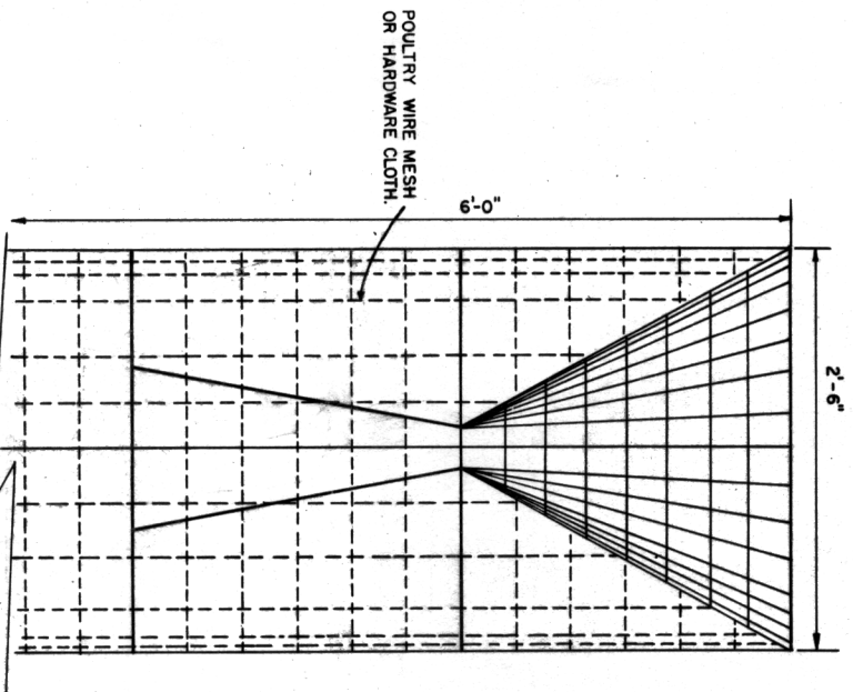
NARROW-MOUTHED FUNNEL TRAP
