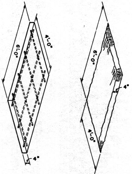
REINFORCED CONCRETE SLAB
