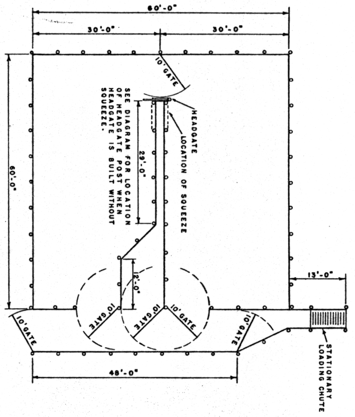
PLAN NO. 1 WITH INTERIOR WORKING CHUTE
