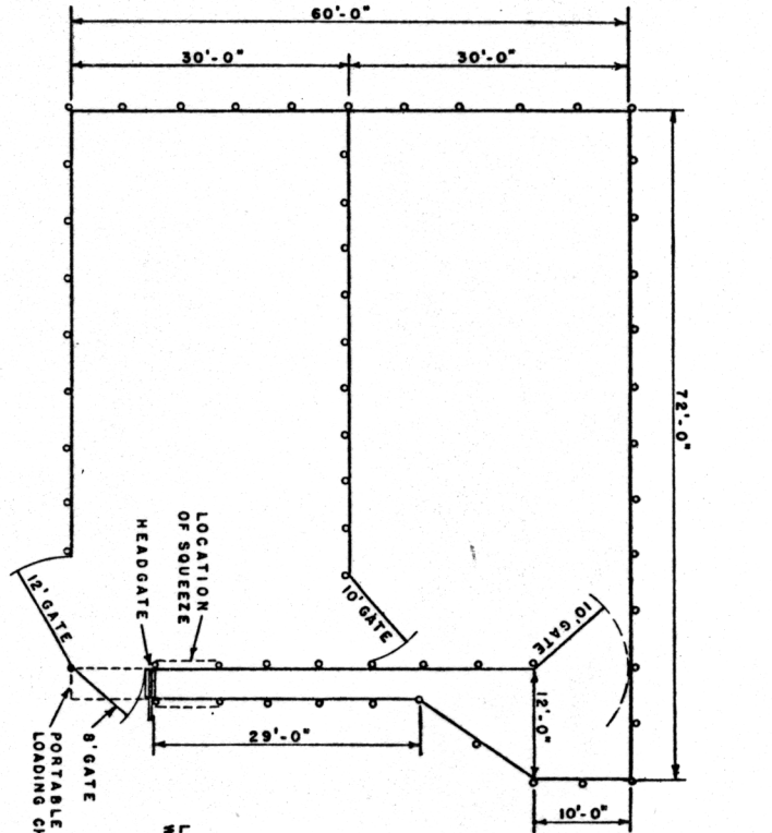
PLAN NO. 2 WITH OUTSIDE WORKING CHUTE
