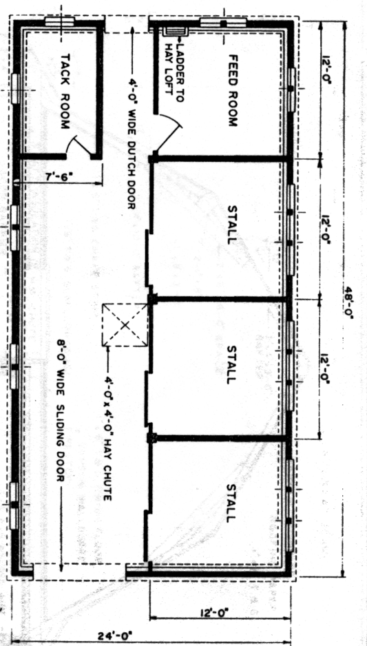
PLAN
