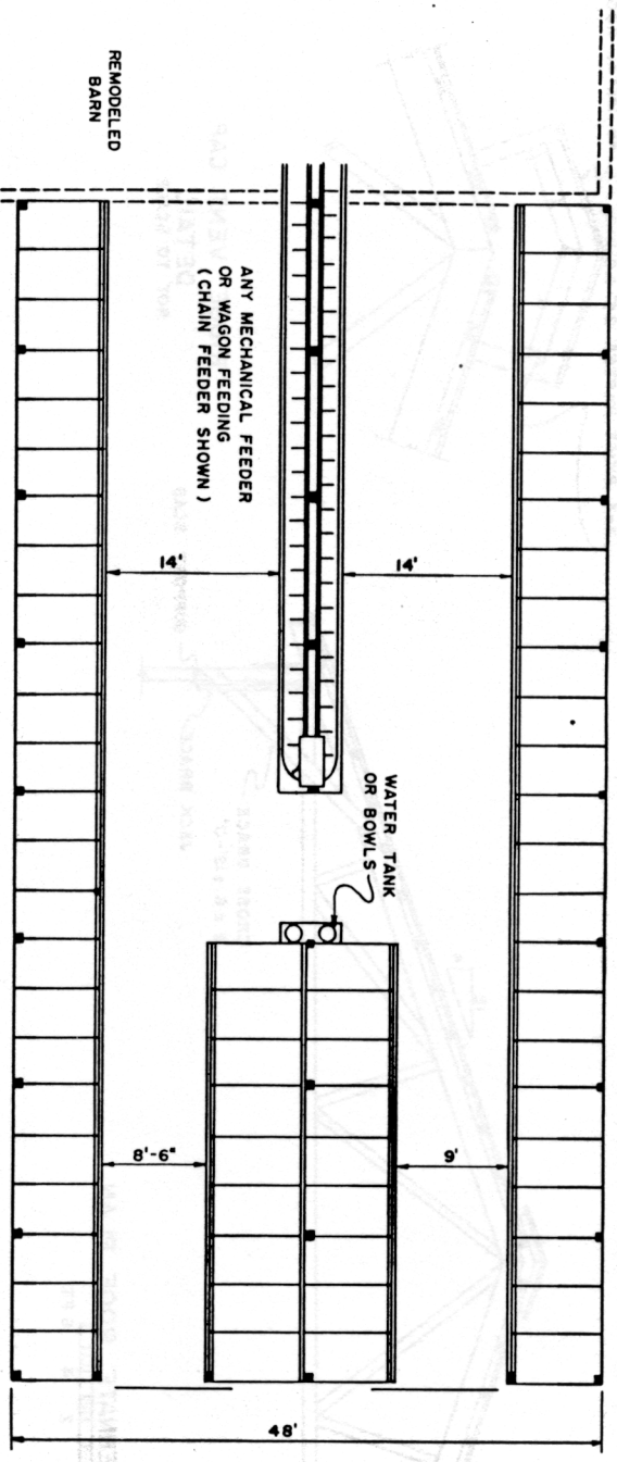
48' BARN FOR FOUR ROWS OF FREE STALLS CENTER FEEDER IF DESIRED
