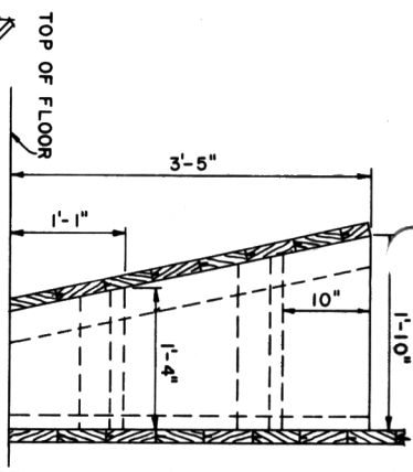
SECTION B-B
