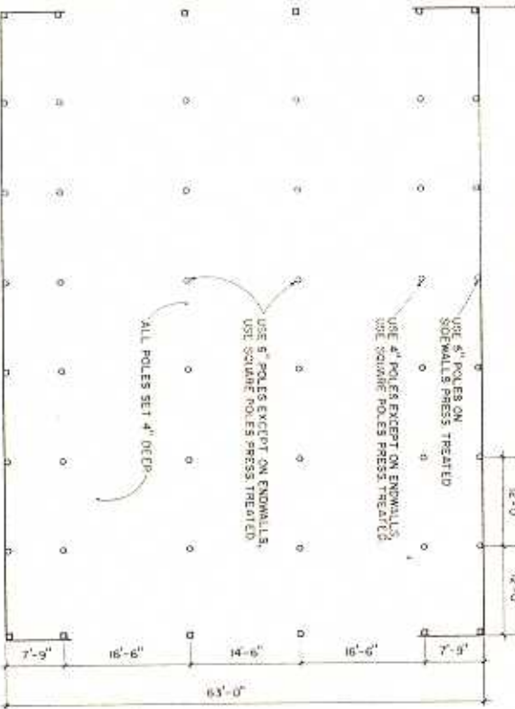
FLOOR PLAN SCALE 1" = 8'-0"
