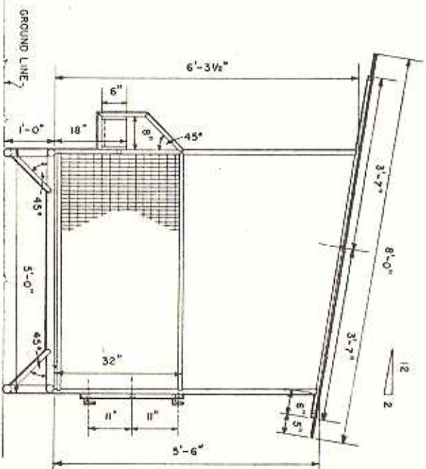
END VIEW SCALE 0 1 2 FT.
