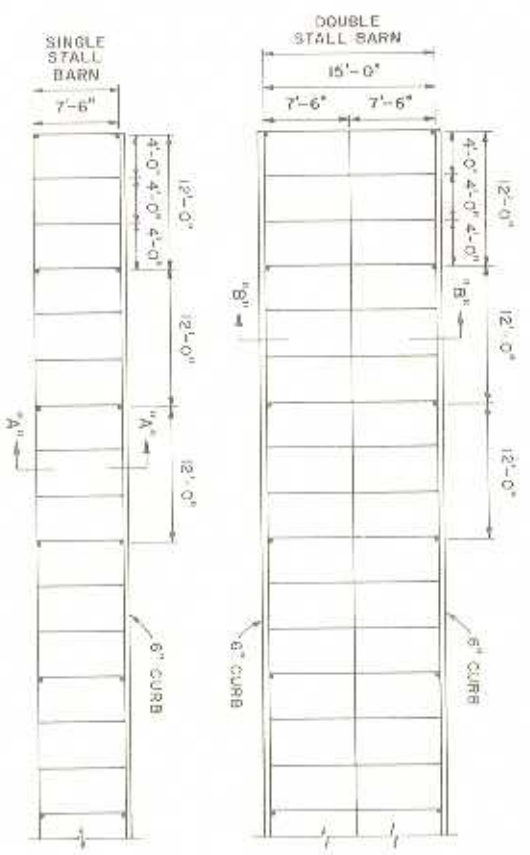
PLAN-SINGLE AND DOUBLE STALL BARN
