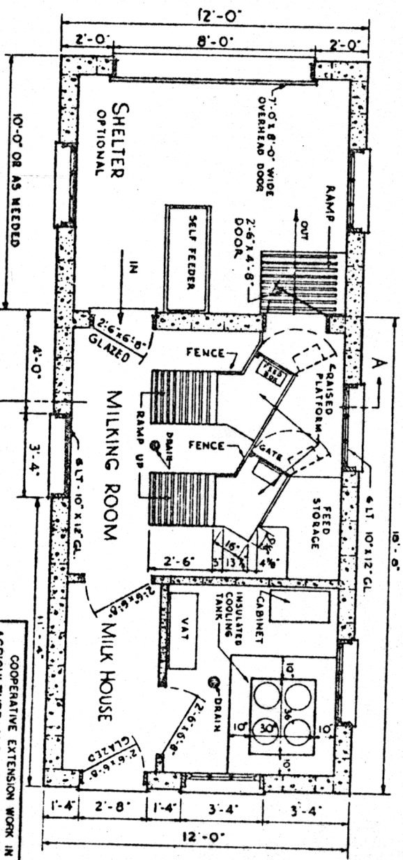
MILKING PLATFORM
