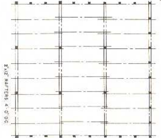
RAFTER LAYOUT SCALE: 1/2" = 4'
