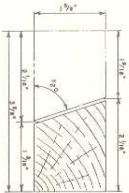
CORNER POST DETAIL RIP FROM DRESSED 2 x 4 SCALE: FULL SIZE
