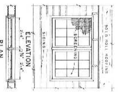
DETAILS OF SASH SCALE 0 1 FT
