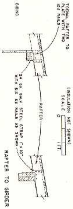
RAFTER TO PLATE
