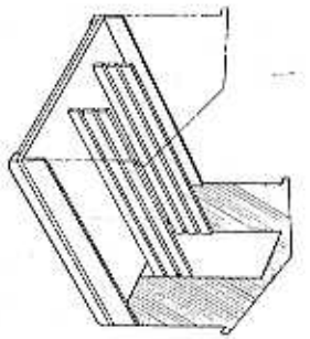
FARROWING STALL FOR 9 SPACES FOR PIGS
