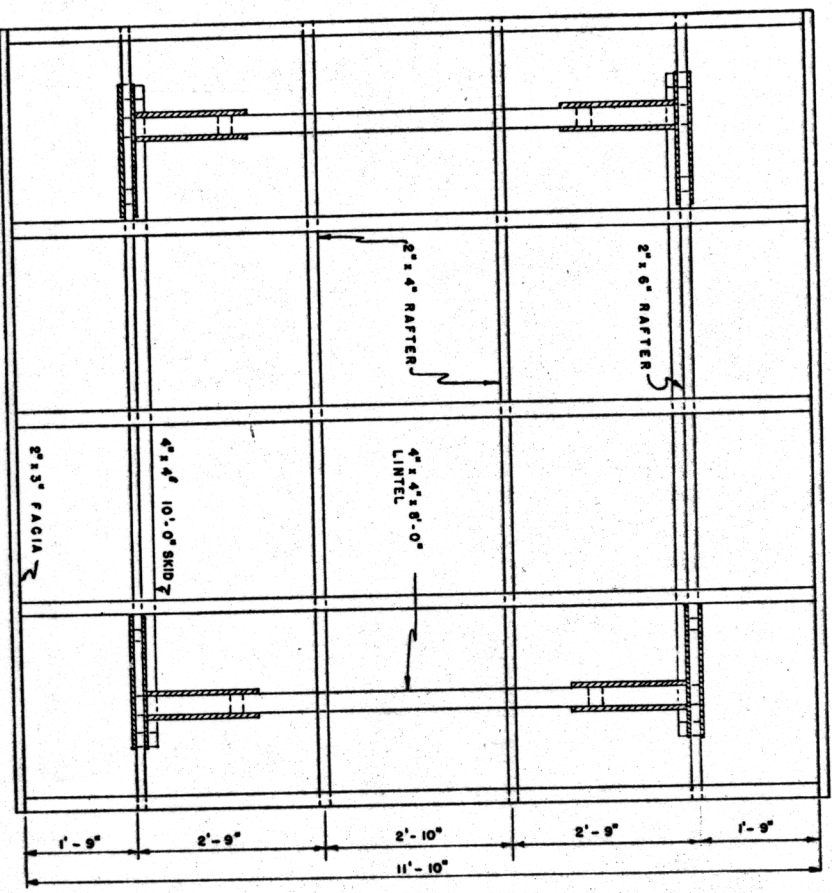
PLAN VIEW OF FRAMING
