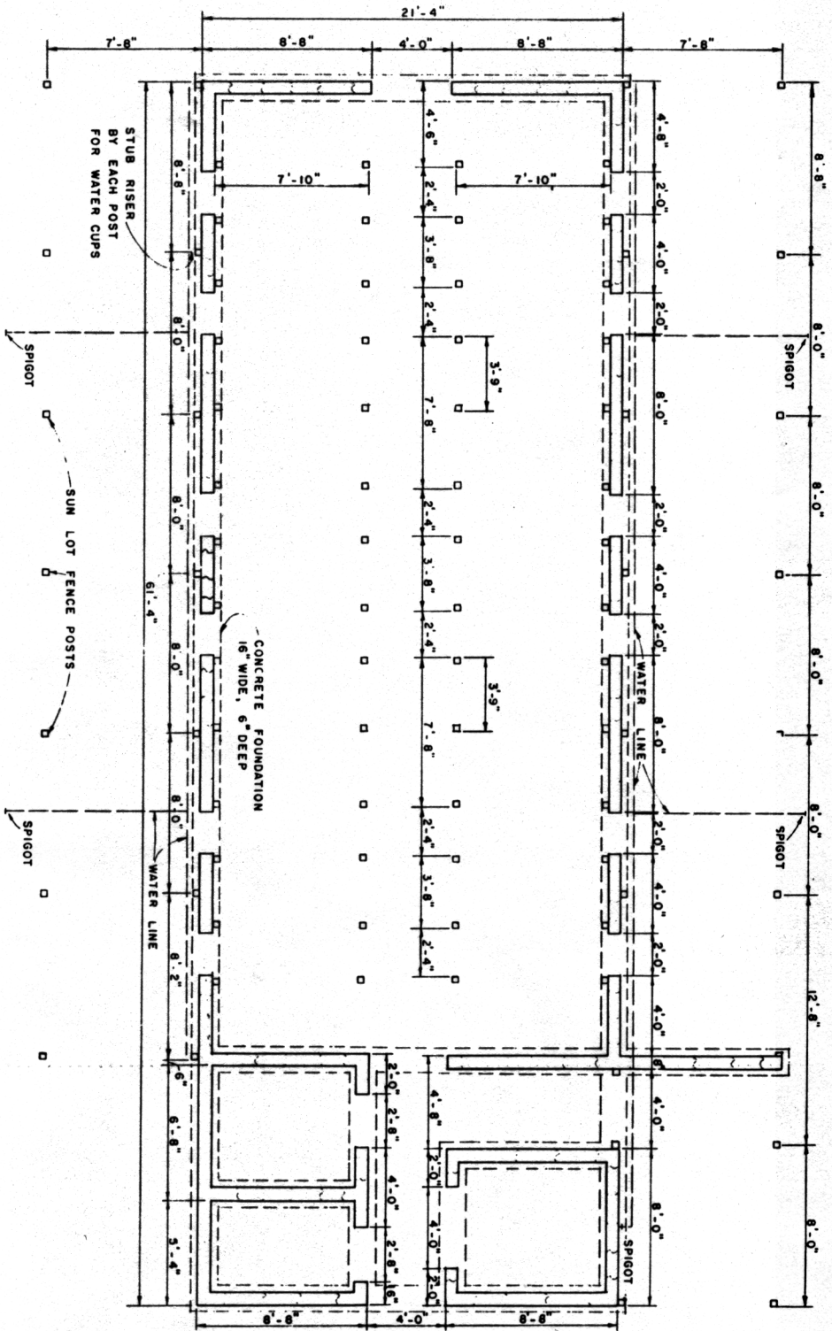
POST B FOUNDATION PLAN
