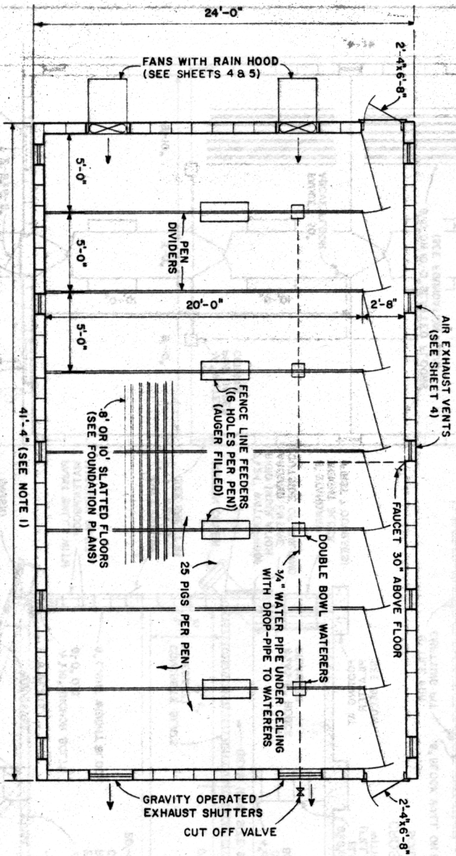
FLOOR PLAN
