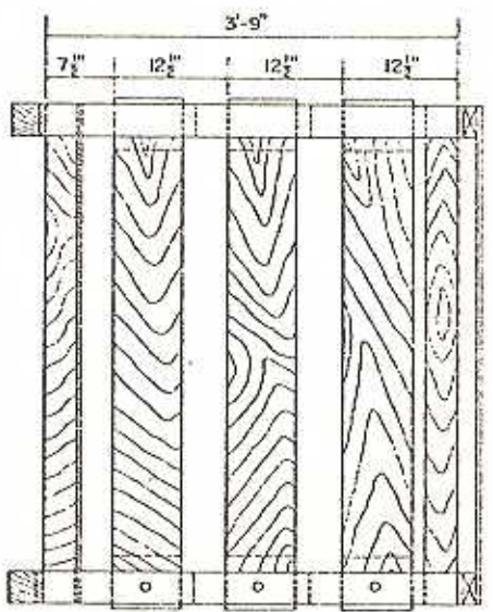
ELEVATION-GATED END
